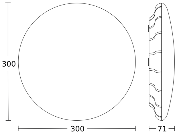
Dimension Drawing 1
